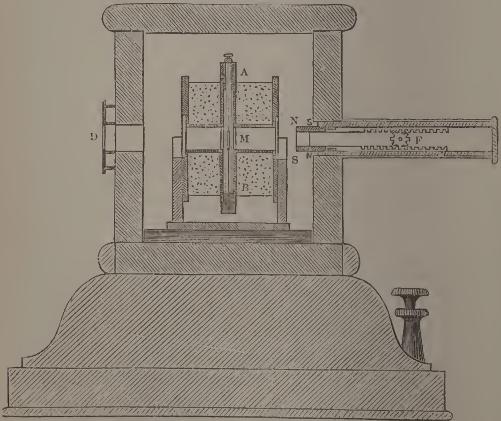
FIG. 98. Sectional Elevation.
